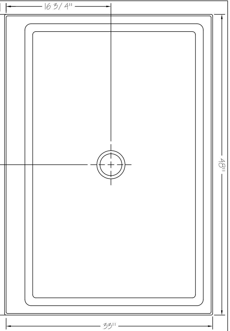
PLAN VIEW
