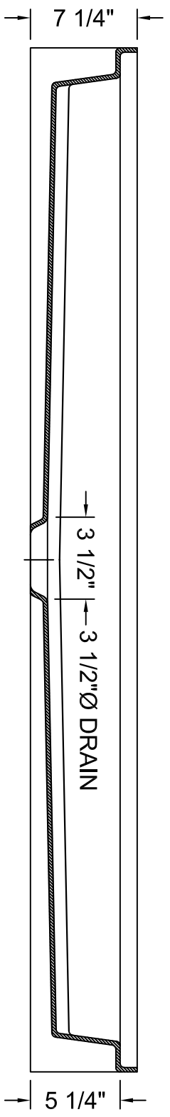
SIDE SECTION
