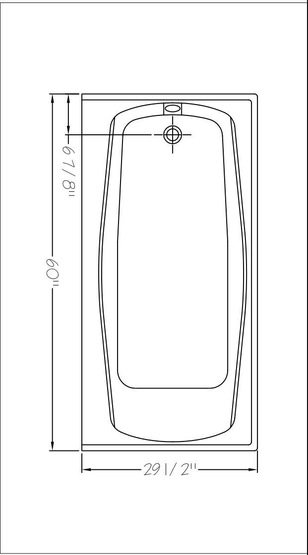
PLAN VIEW
