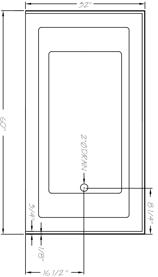
PLAN VIEW
