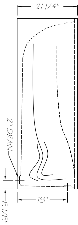
FRONT ELEVATION
