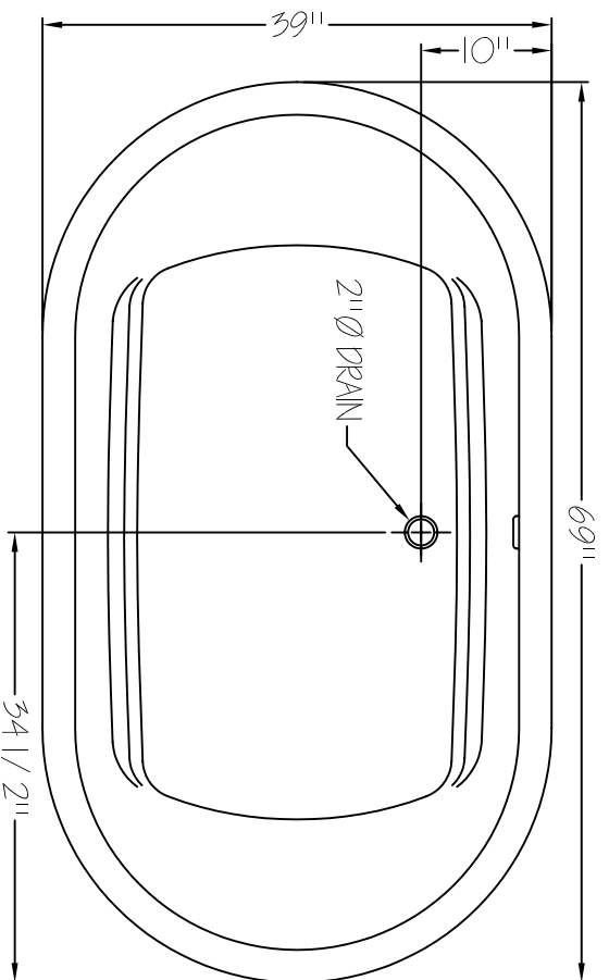
PLAN VIEW
