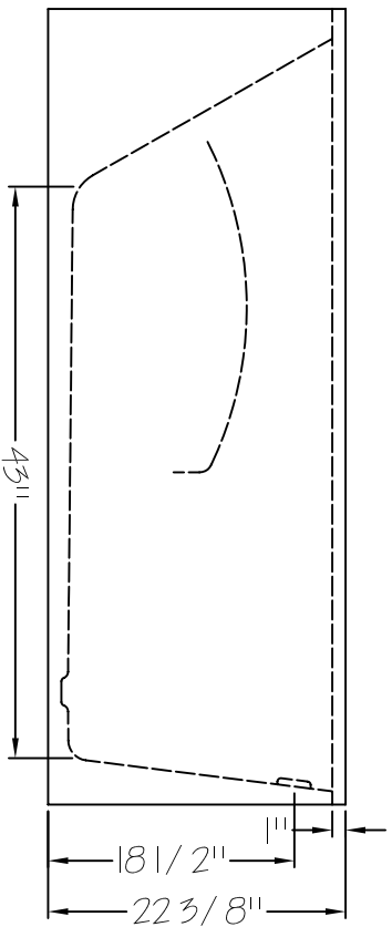
PLAN VIEW
