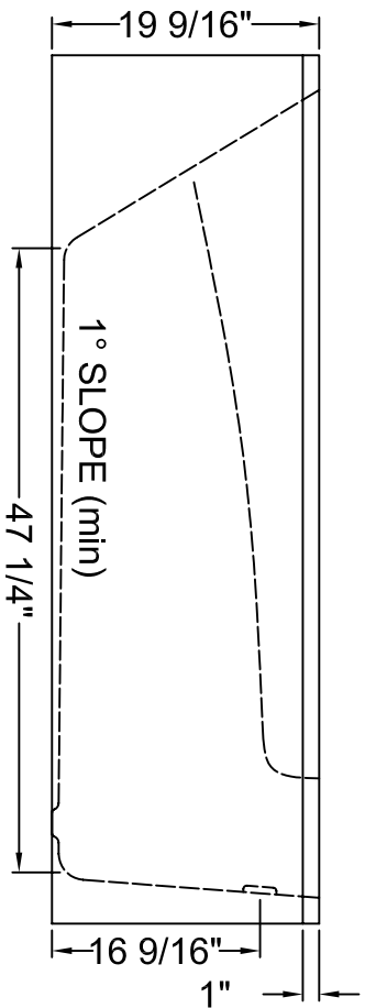
FRONT ELEVATION
