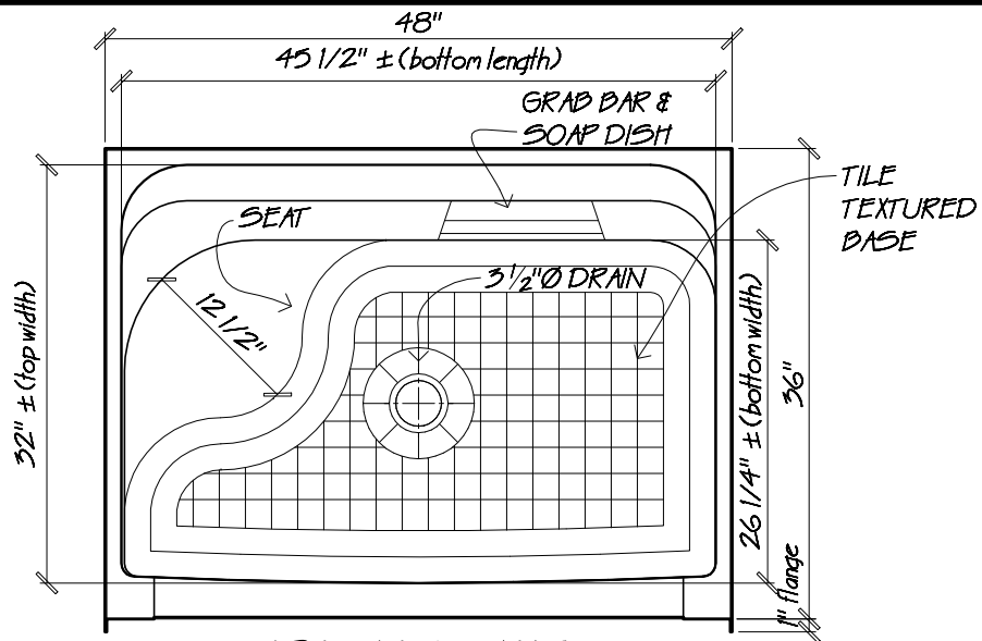
PLAN VIEW
