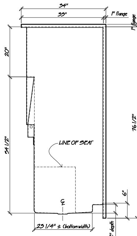
LEFT END VIEW scale: 1/2" = 1"
