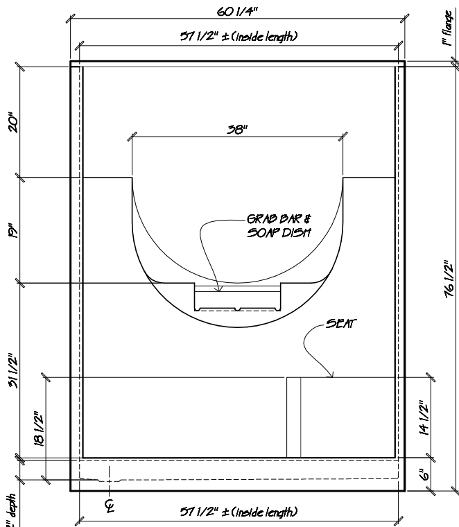
FRONT VIEW scale: 1/2" = 1"
