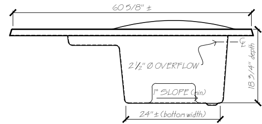
END VIEW
