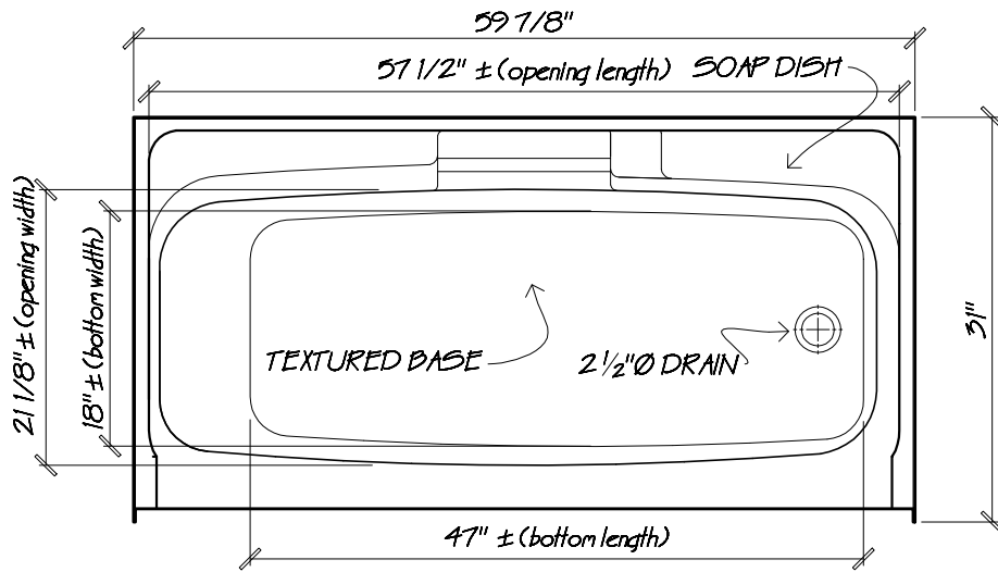
PLAN VIEW scale: 3/4" = 1"
