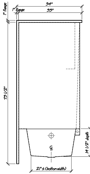
RIGHT END VIEW scale: 1/2" = 1"
