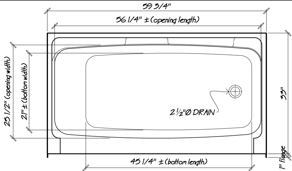
PLAN VIEW scale: 3/4" = 1"
