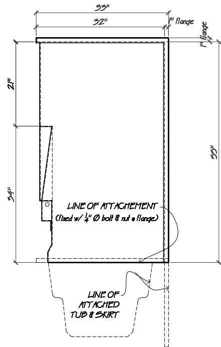
RIGHT END VIEW scale: 1/2" = 1"
