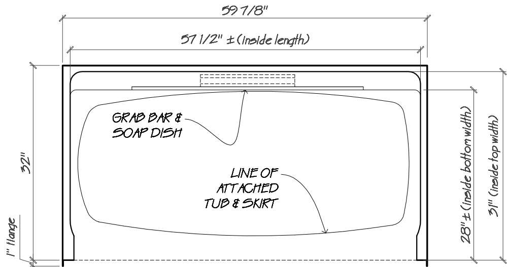
PLAN VIEW scale: 3/4" = 1"
