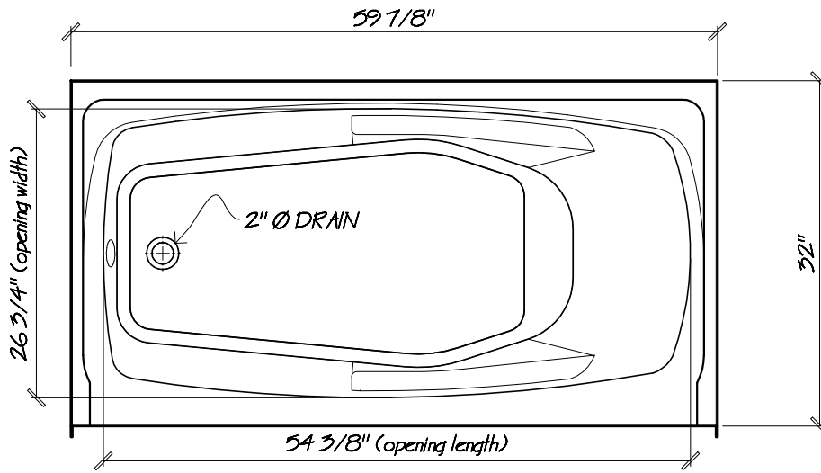
PLAN VIEW
