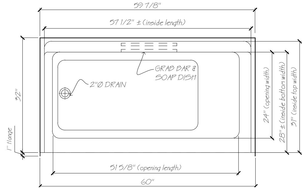
PLAN VIEW scale: 3/4" = 1"
