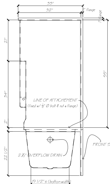
RIGHT END VIEW scale: 1/2" = 1"
