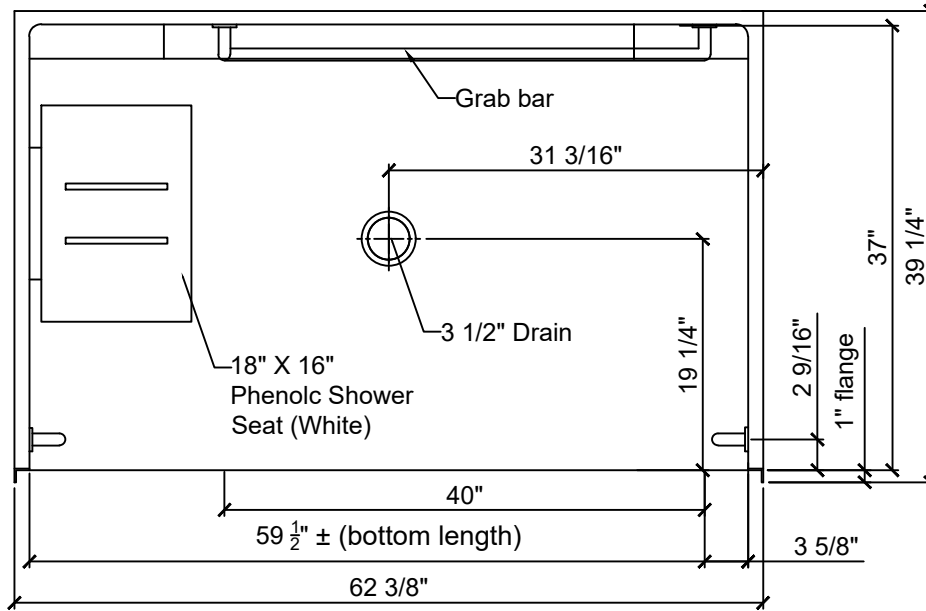
PLAN 1' - 0' 3/4"
